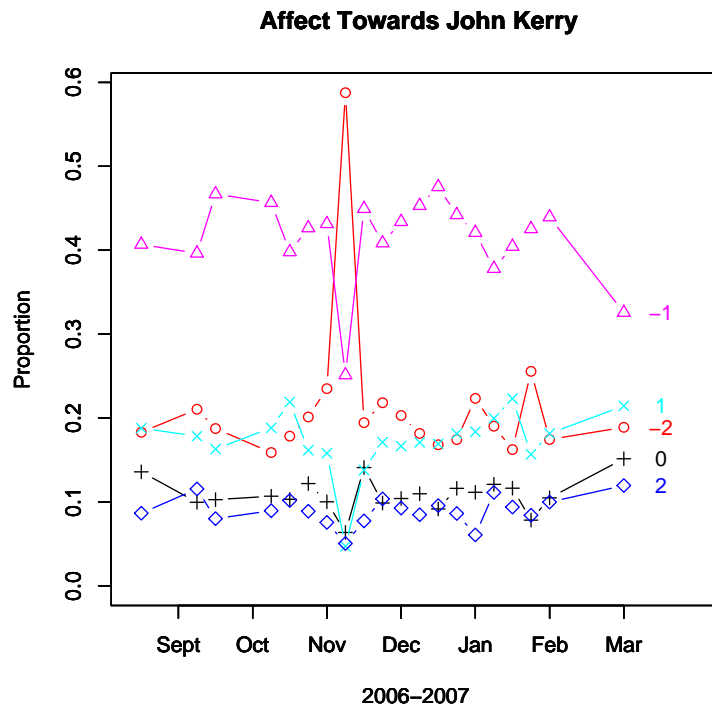
Figure 1: Blogosphere Responses to Kerry’s Botched Joke. Each line gives a time series of estimates of the proportion of all English language blog posts in categories ranging from -2 (extremely negative, colored red) to 2 (extremely positive, colored blue). The spike in the -2 category immediately followed Kerry’s joke. Results were estimated with our nonparametric method in Section 5.2.
