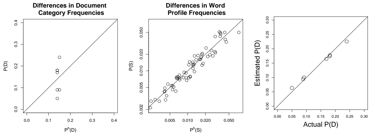
Figure 2: Accurate Estimates Despite Differences between Labeled and Population Sets: For both P(D) on the left and P(S) in the center, the distributions differ considerably. The direct sampling estimator, P^h(D) , is therefore highly biased. Yet, the right panel shows that our nonparametric estimator remains unbiased.
