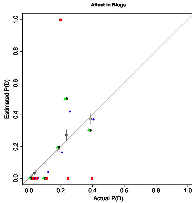
Figure 3: Out-of-sample Validation. The plot gives the estimated document category frequencies (vertically) by the actual frequencies (horizontally). Our nonparametric approach is represented with black open circles, with 95% confidence intervals as vertical lines. Aggregated optimized SVM analyses also appear for radial basis (black dots), linear (green triangles), polynomial (blue diamonds), and sigmoid kernels (red squares). Estimates closer to the 45^\circ line are more accurate.
