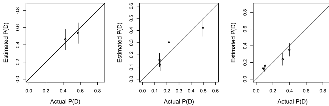
Figure 4: Additional Out-of-sample Validation. The left graph displays the accuracy of the nonparametric method in recovering the distribution of supporting versus opposing speeches in Congress. The center graph shows the same for a categorization of newspaper editorials on immigration, and the right graph shows the distribution across categories of emails sent by Enron employees. As before, 95% confidence intervals are represented by vertical lines, and estimates closer to the 45° line are more accurate.
