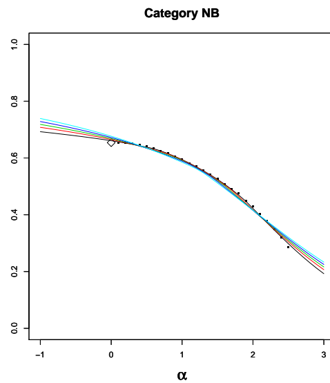
Figure 6: SIMEX Analysis of the Proportion of documents in Category NB (not a blog). The estimate from the observed data appears above 0 marked with a diamond; other points are simulated. The goal is to decide on the proportion in category NB at a horizontal axis value of -1 .
